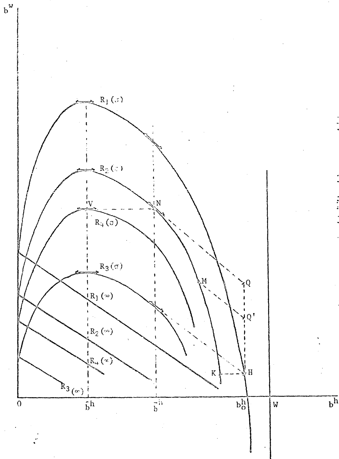
Figure 2: Iso-interest Contours
